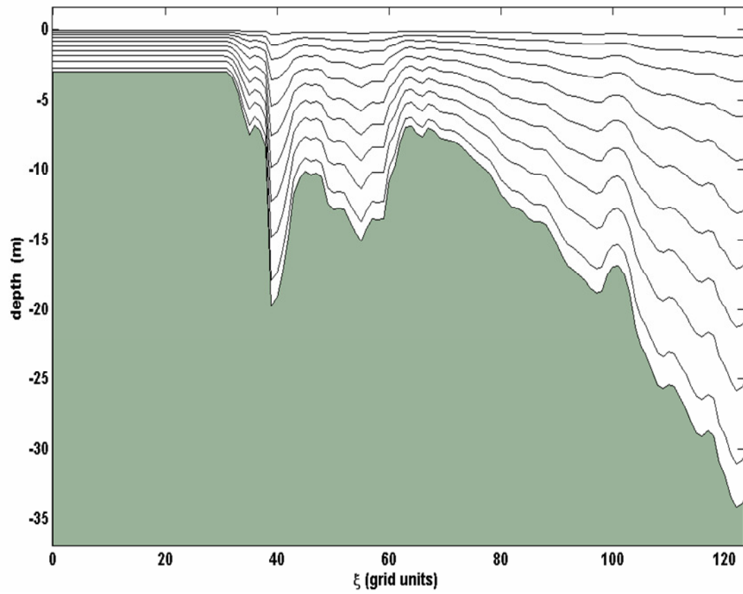
Figure 2.5 Different vertical levels for a horizontal slice through the grid at \eta = 205 . Notice how at the top level the elevation is very close for all points, regardless of depth.
